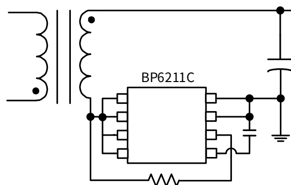
Figure 1. BP6211C Typical Application
